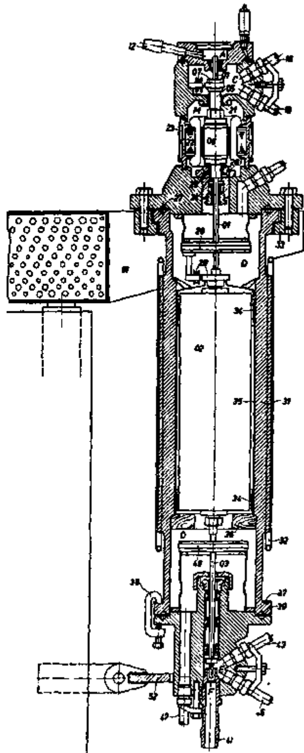
Figure 1 The Present German 300 Meter-Per-Second Gas Centrifuge
