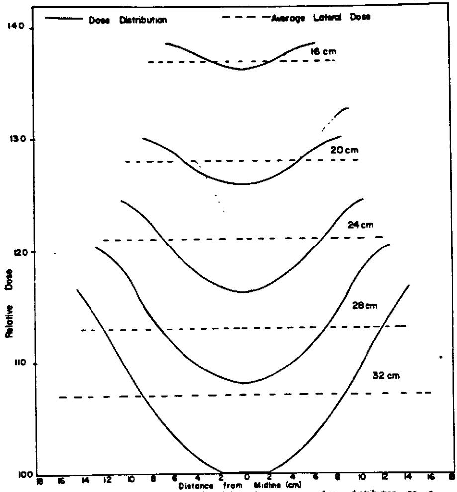
Figure 3 Dose distribution for bilateral exposure, dose distribution as a function of lateral thickness for a given midline exposure.
